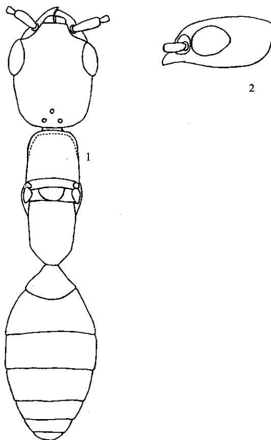
Figs. 1-2 Bethylus sinensis Xu, He et Terayama, sp. nov. 中华肿腿蜂, 新种 1. Body, dorsal view 体背面观; 2. head, lateral view 头部侧观
